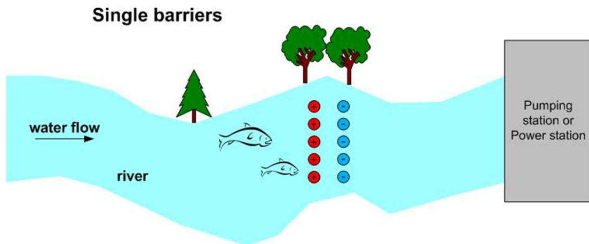
Figure 4-1 Arrangement of the NEPTUN Electric Fish Barrier at an Intake (Courtesy of PROCOM Systems)
