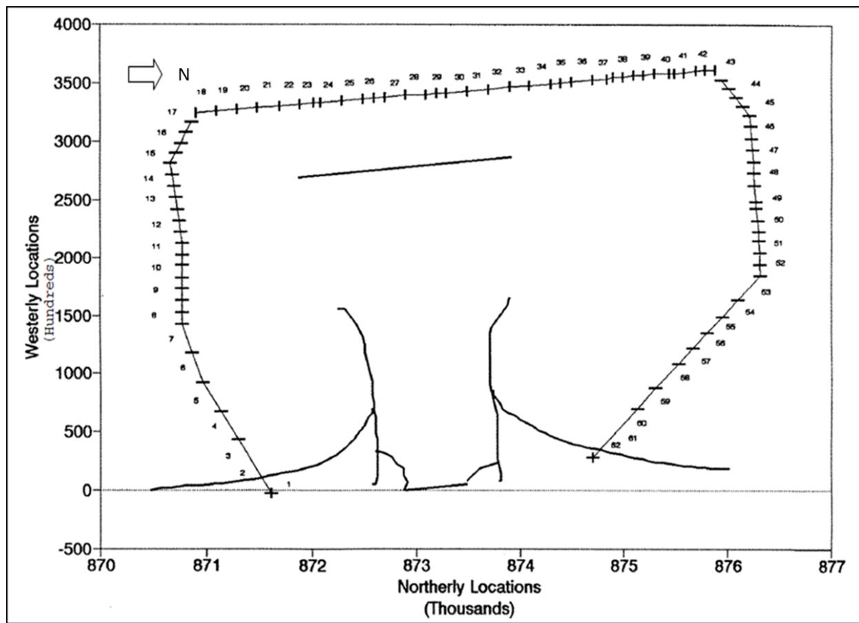
Figure 4-1: Overview of Primary Net Sections and Panels at LPS
