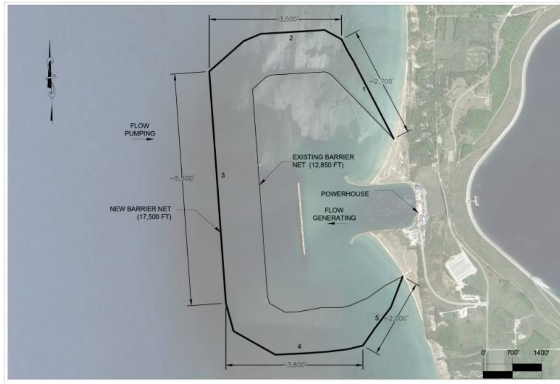
Figure 7-3: New longer barrier net with ½-inch bar mesh – plan
