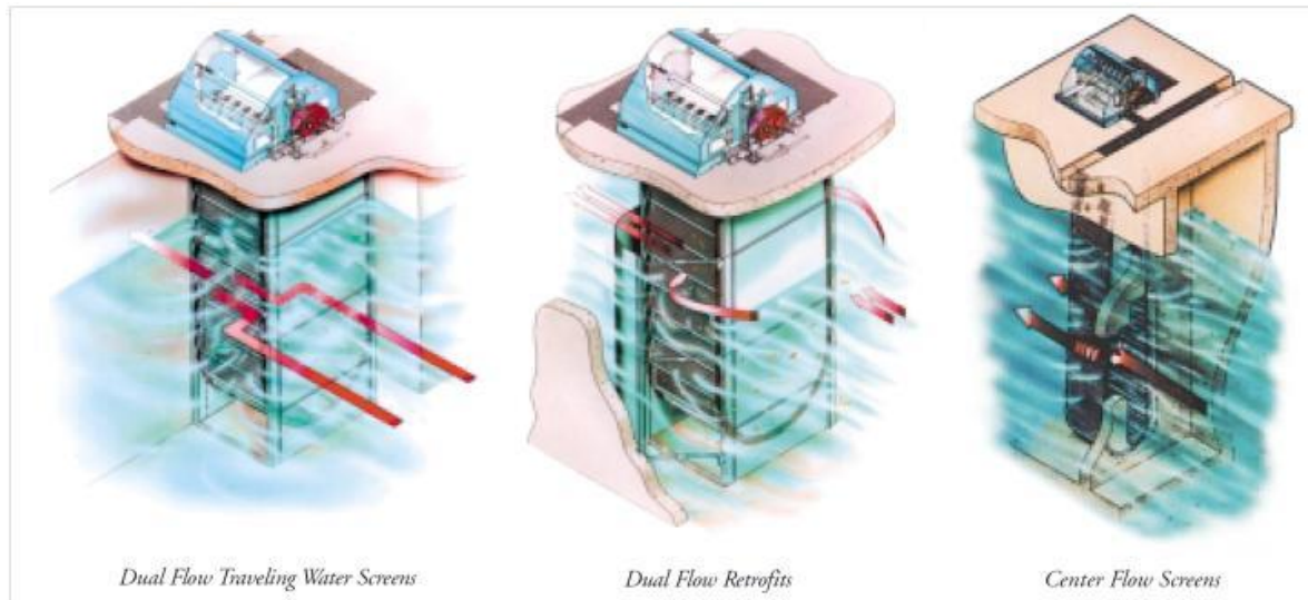
Figure 4-16 Various Types of Traveling Water Screens (Courtesy of U.S. Filter 3 )
